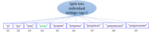
Figure 1: A word split into incremental substrings
