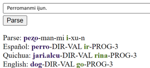
Figure 3: RB-based parser output
